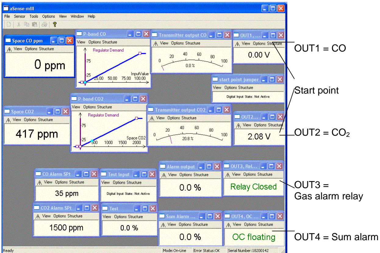
Figure 2 Print screen of UIP4.3 PC work space of CF8-W-Disp-CO where the pre-set functions can easily be redefined. The four outputs (far right) are here arranged in rows together with the function blocks that control the output.
