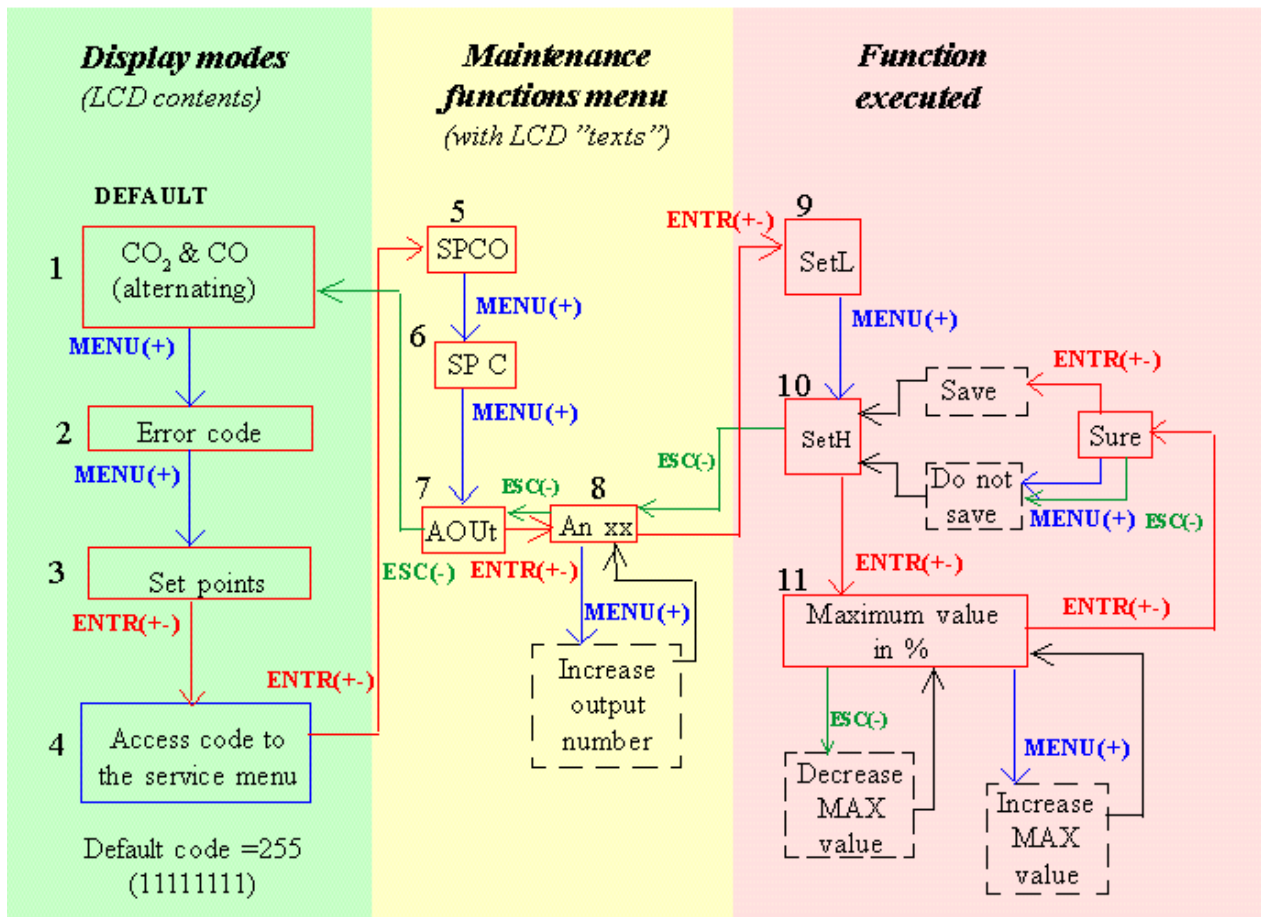
Figure 10 Maintenance functions available on CF8-W-Disp-CO to set output limits. Only flow chart for setting High limits is shown, but Low limits are set in the very same way. The numbers in the flow chart refers to the points in example 1. Function blocks that are time limited are indicated by blue boards. Time limit refers to an internal time-out that returns the LCD and maintenance function back to normal. ENTER is a simultaneous pressing on MENU and ESC.
