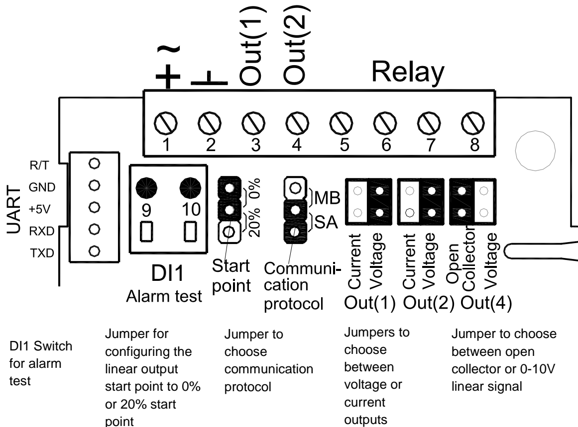
Figure 5 The connection terminal area of the CF8-W-Disp-CO with jumpers and terminals. The terminal DI1 may be used for forced ventilation. If the sensor has a heater it is connected to \sim and \pm .
