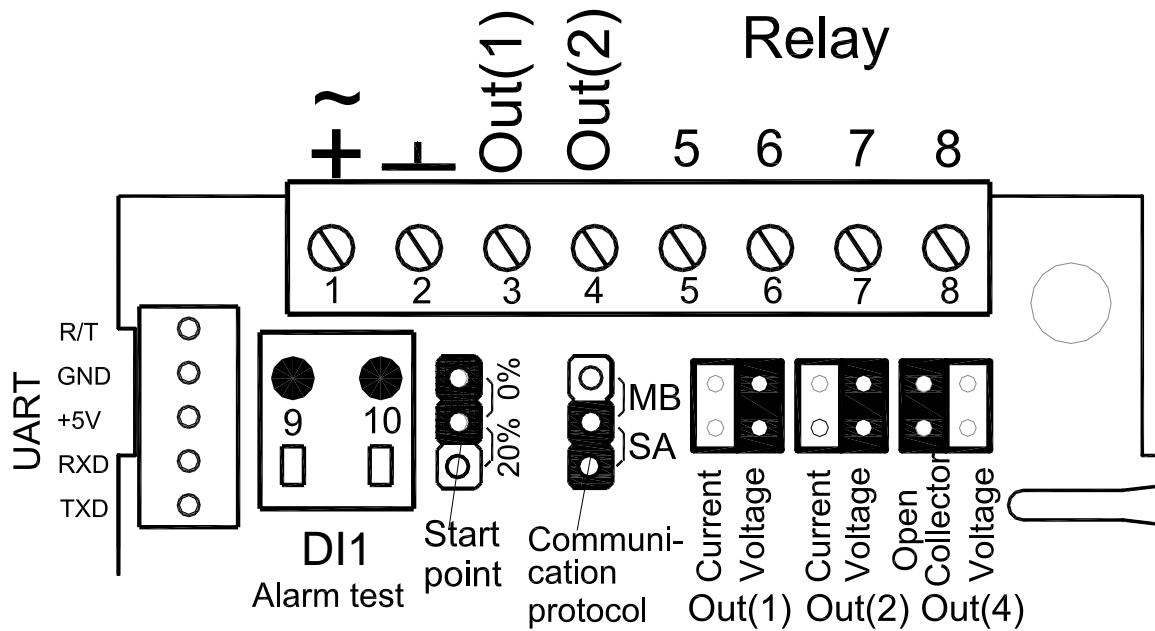
Figure 12. The CF8-W-Disp-CO printed circuit board with the connection terminal area is enlarged. The terminal DI1 may be used for forced ventilation. If the sensor has a heater it is connected to \oplus and \ominus .
